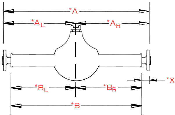
HOUSING
