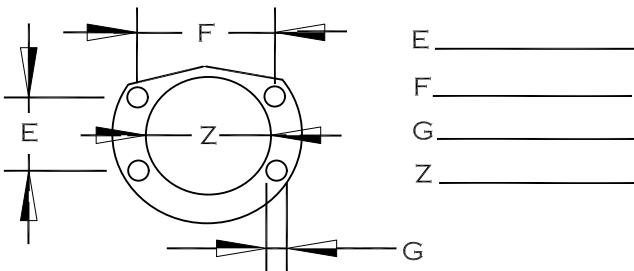
HOUSING FLANGE
