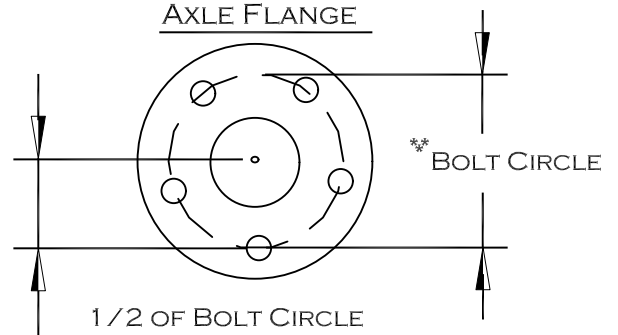
AXLE FLANGE
