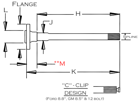
AXLE
